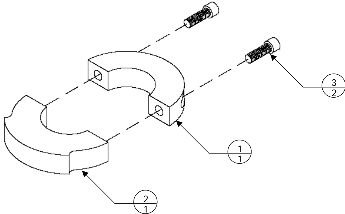
Part No. 9101179A (OCR / SELECTIVE CAM ASSEMBLY)
