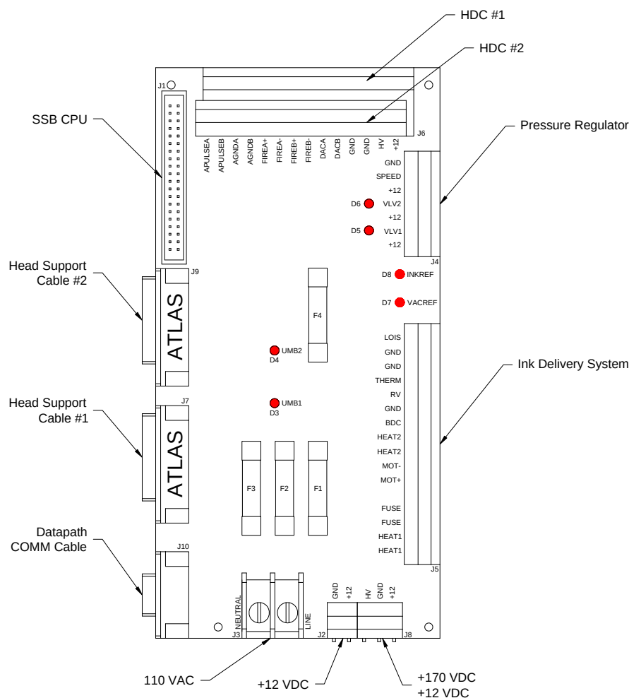
Figure 2-1: Atlas System Support Board
