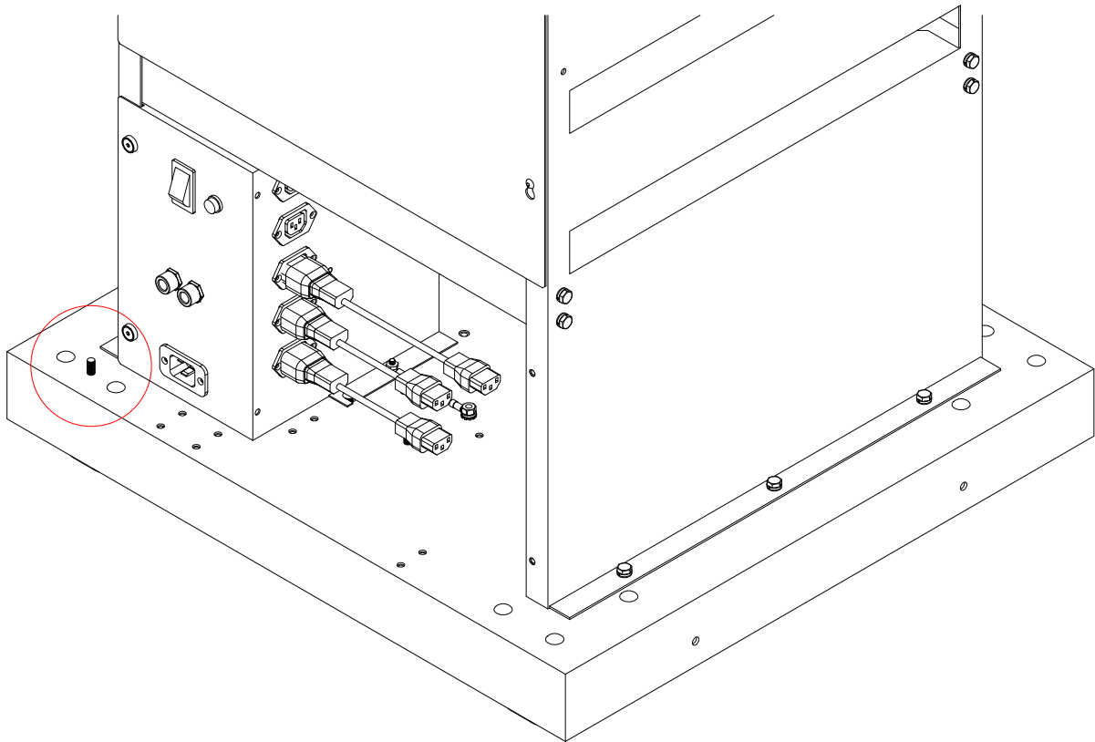
Figure 2-18: BK705 Ground Stud
