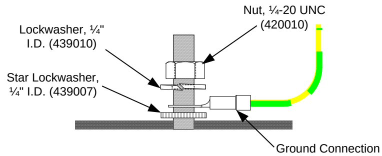
Figure 2-19: Ground Stud
