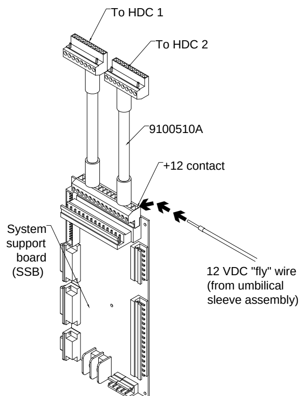
Figure 2-4: Cable connections for 2250 on SSB
