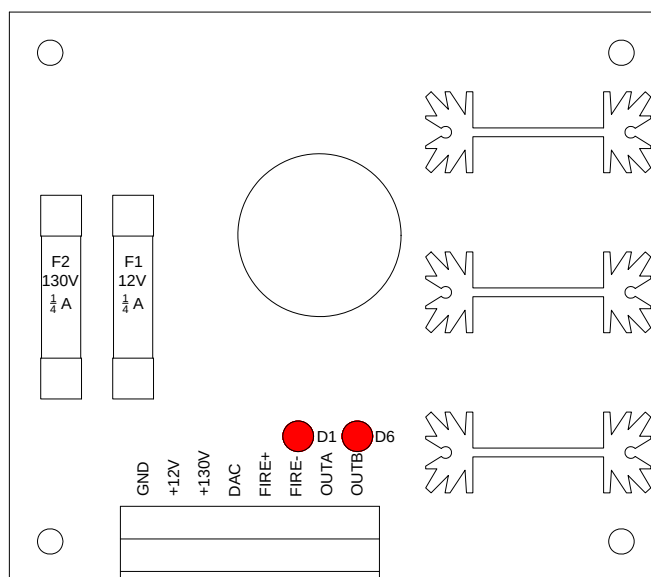
Figure 2-3: Head Drive Circuit Board
