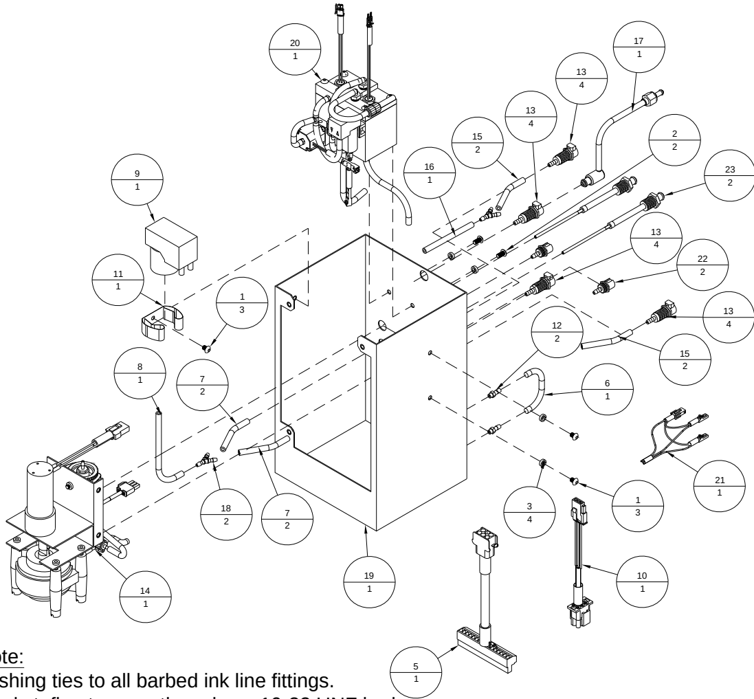
Figure B-21: 9103766A – Ink Delivery Module, BK705 Atlas (Monet &amp; Cezanne)
