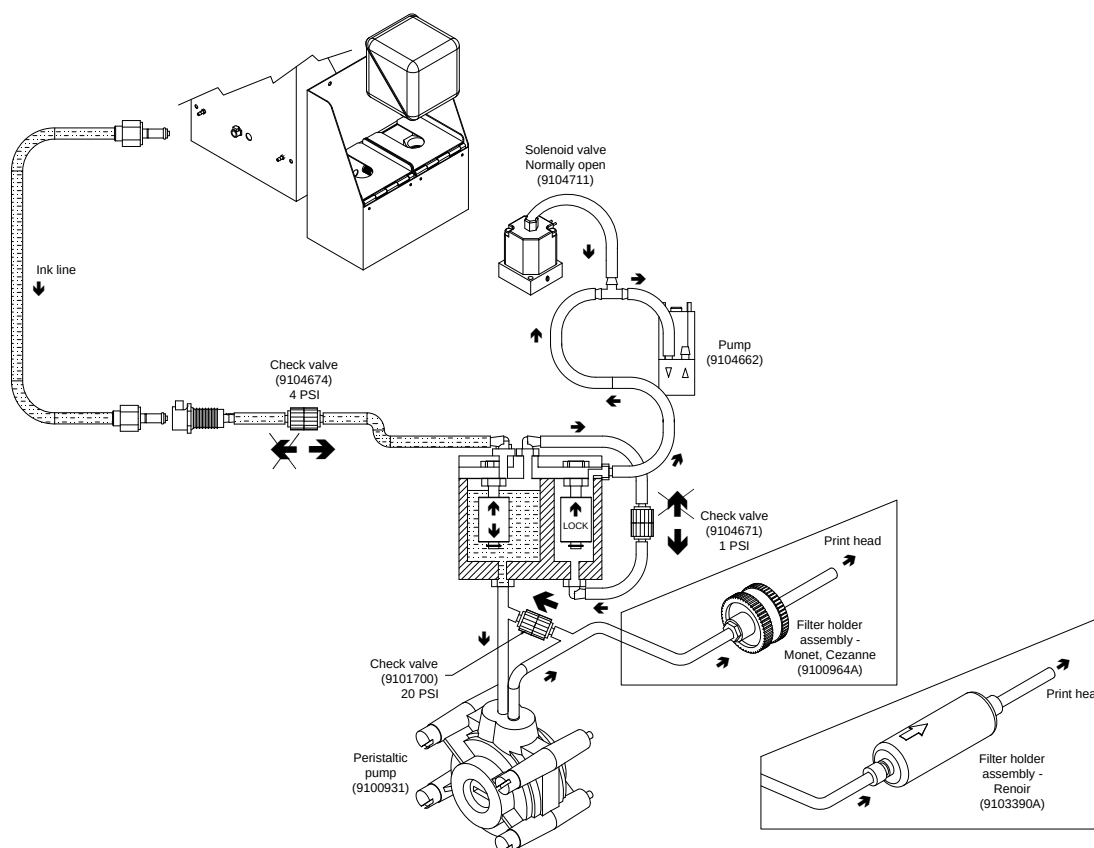
Figure 2-5: Ink Supply Line
