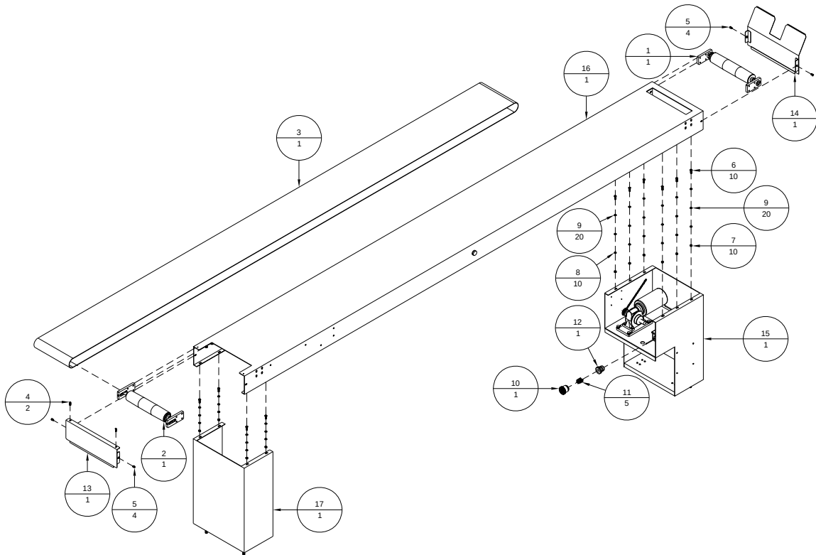
Figure A-12: BK1612ASB - Conveyor Assembly, 12', Solid Belt
