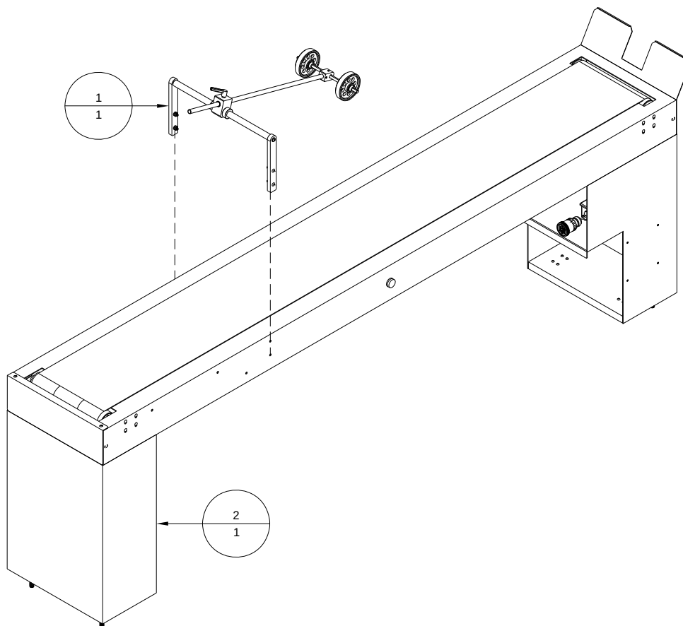
Figure A-2: BK1608SBI - Conveyor, 8' Solid Belt, Inline
