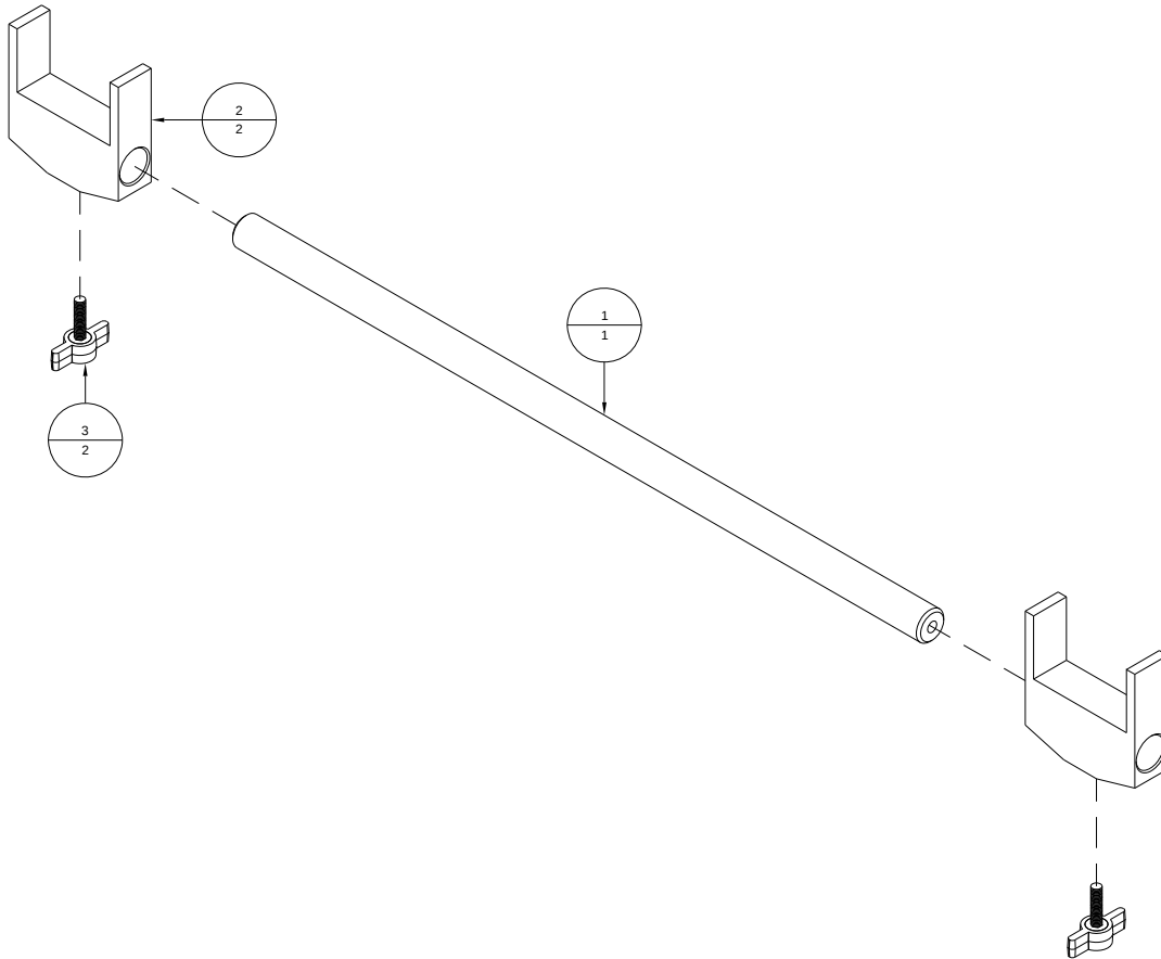
Figure A-17: 100167A - Belt Alignment Assembly, Twin Belt
