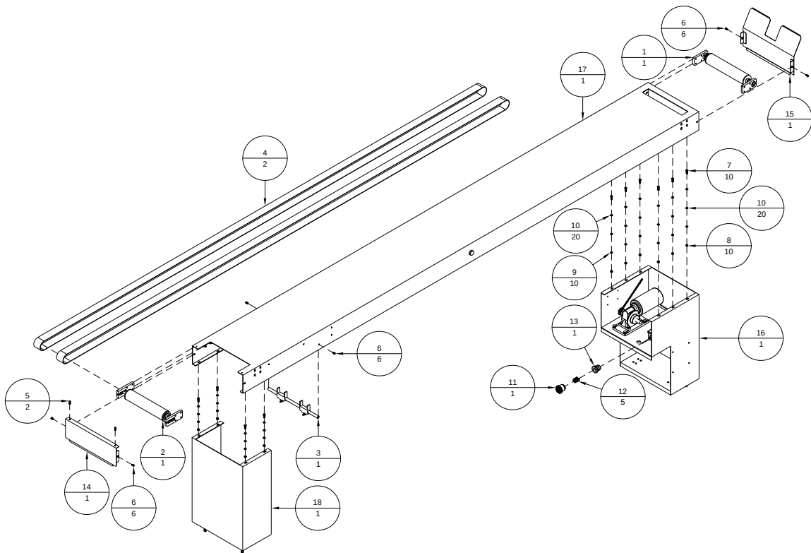
Figure A-11: BK1612A - Conveyor Assembly, 12', Twin Belt
