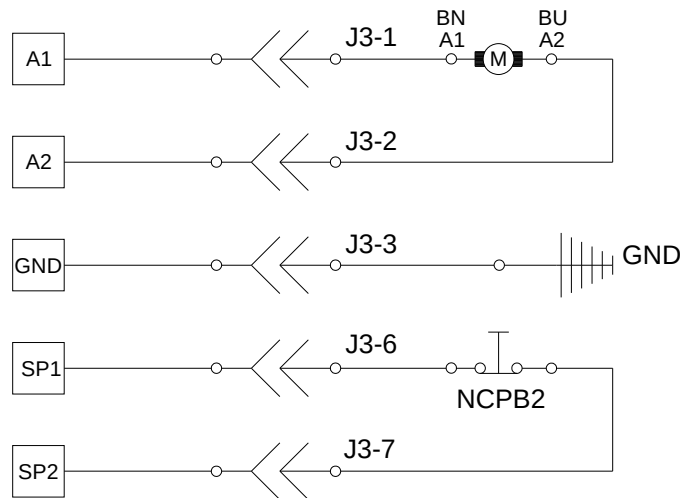
Figure B-1: Electrical Schematic, BK1600 Series Conveyor
