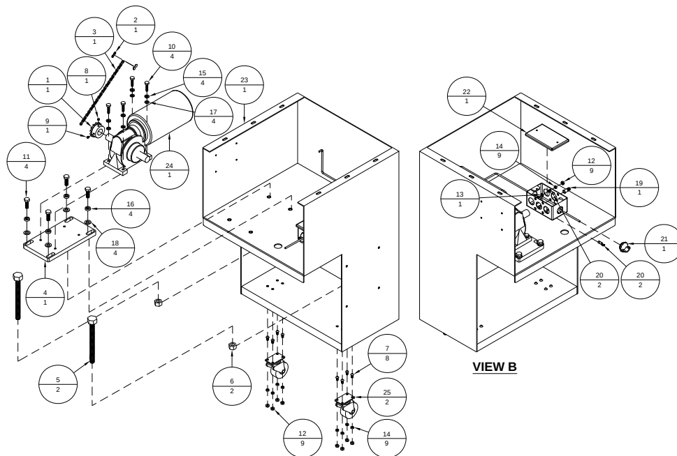
Figure A-23: 706155A – Conveyor Motor Stand Assembly
