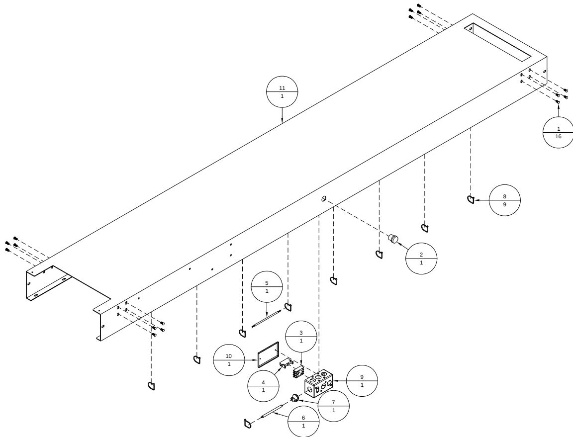
Figure A-24: 706158A - Conveyor Bed Assembly, 8'
