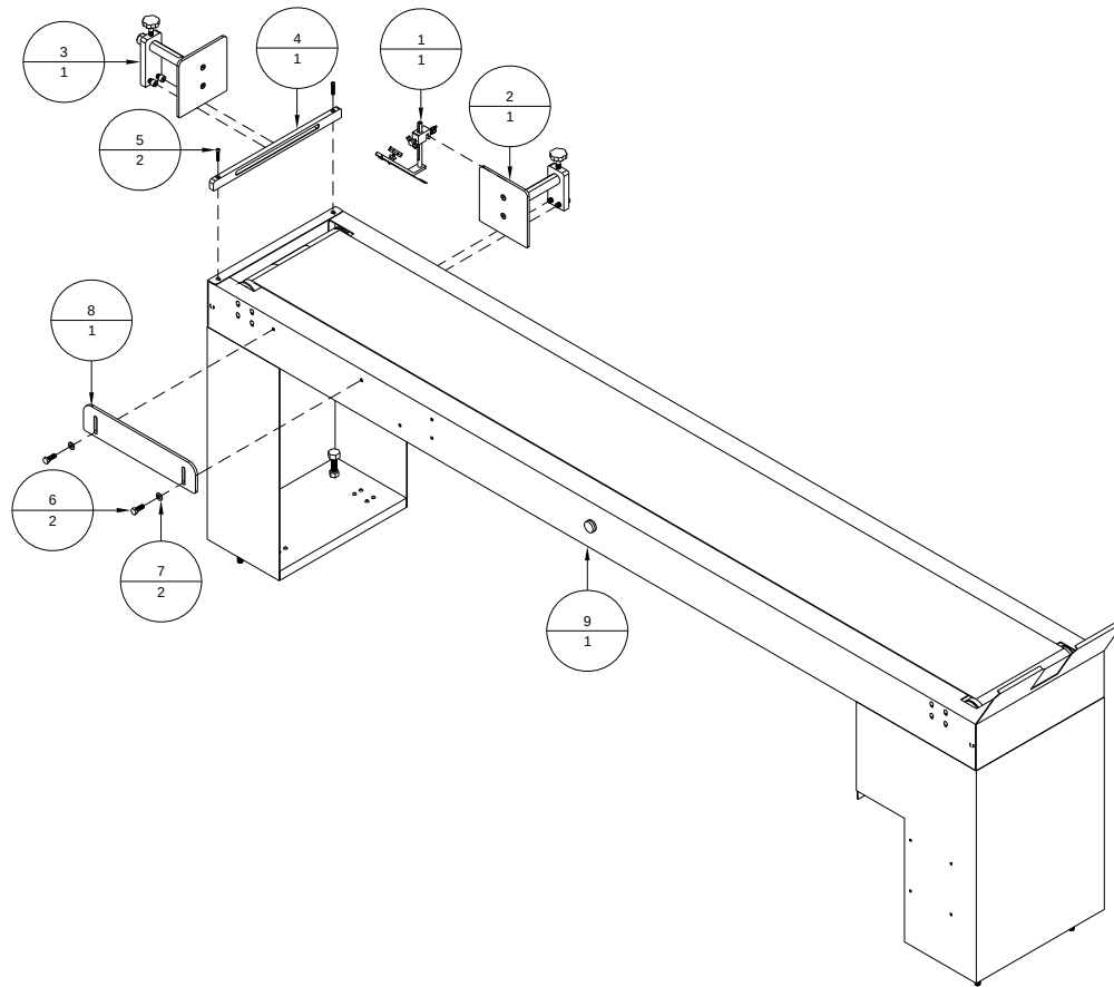
Figure A-1: BK1608SB - Conveyor, 8', Solid Belt, Right Angle
