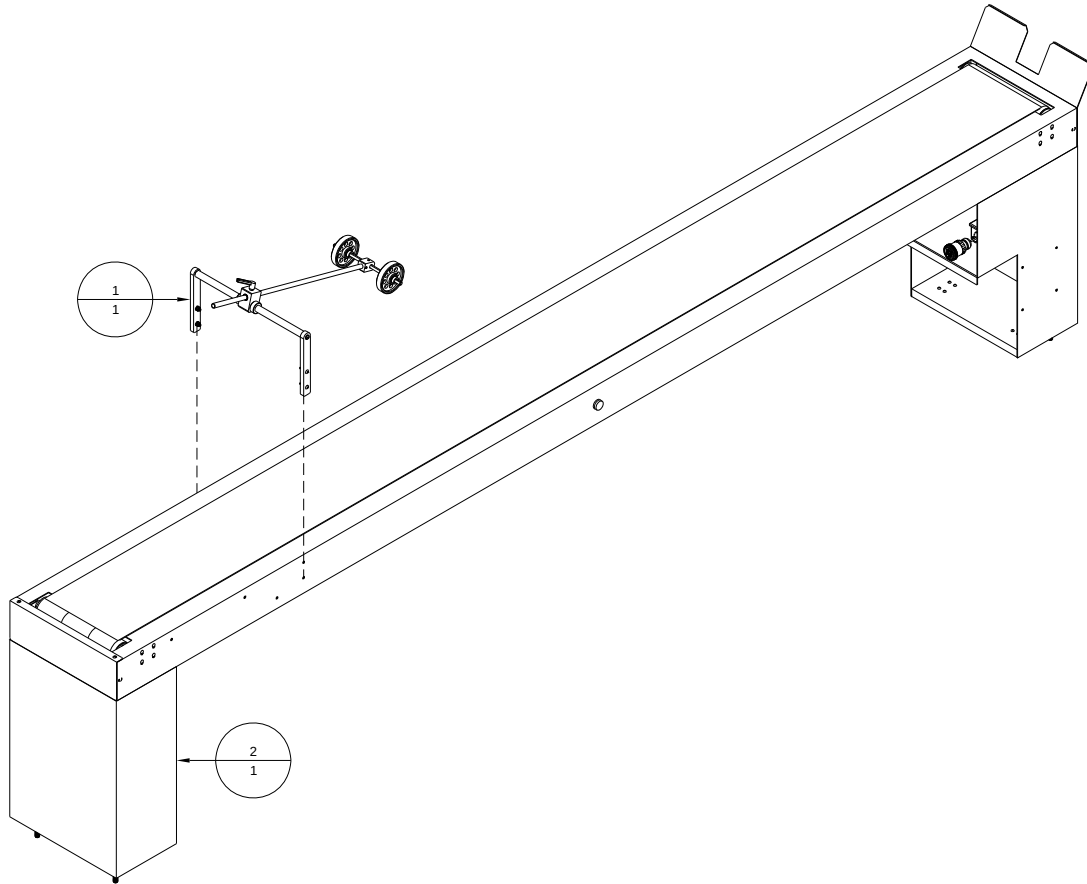
Figure A-6: BK1612SBI - Conveyor, 12' Solid Belt, Inline
