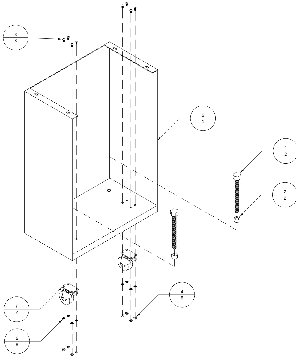
Figure A-26: 706165A – Conveyor End Stand Assembly
