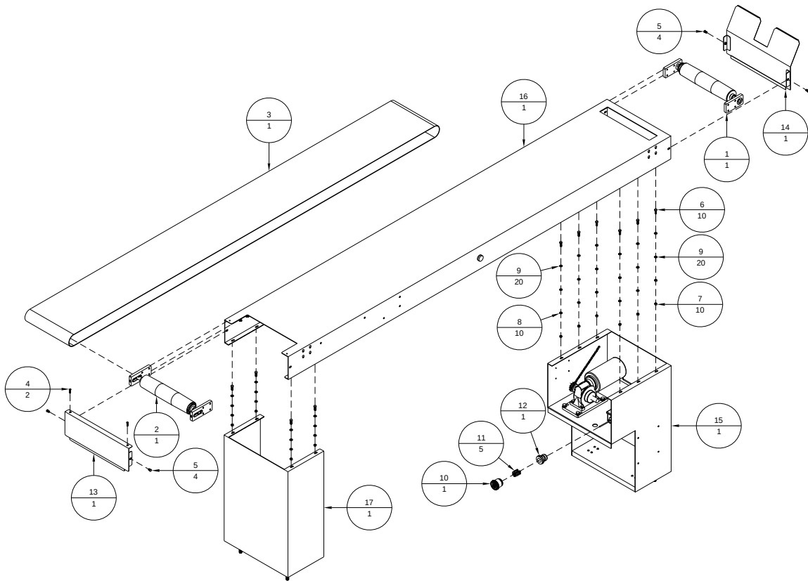
Figure A-10: BK1608ASB - Conveyor Assembly, 8', Solid Belt
