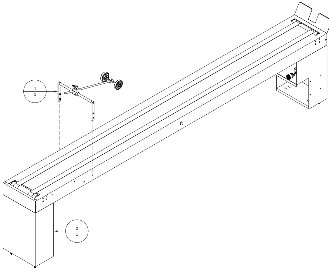
Figure A-8: BK1612TBI - Conveyor, 12' Twin Belt, Inline
