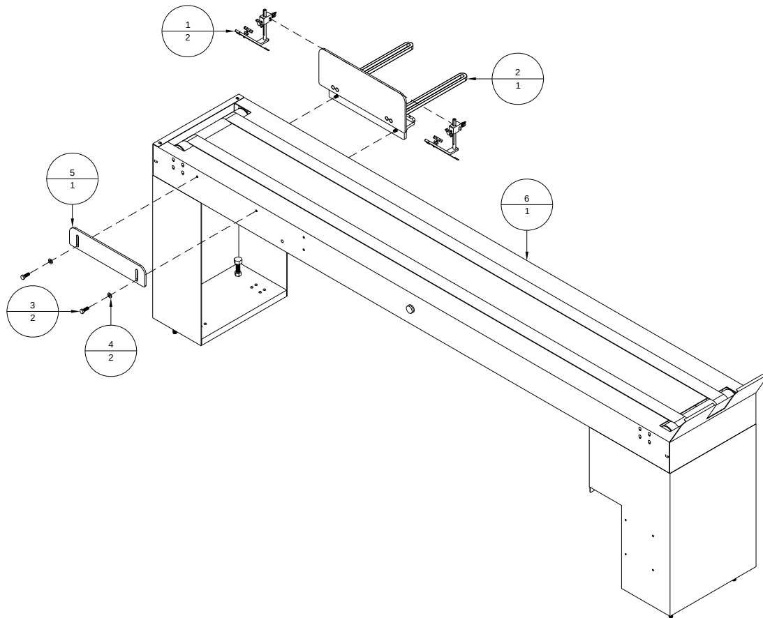
Figure A-3: BK1608TB - Conveyor, 8' Twin Belt, Right Angle
