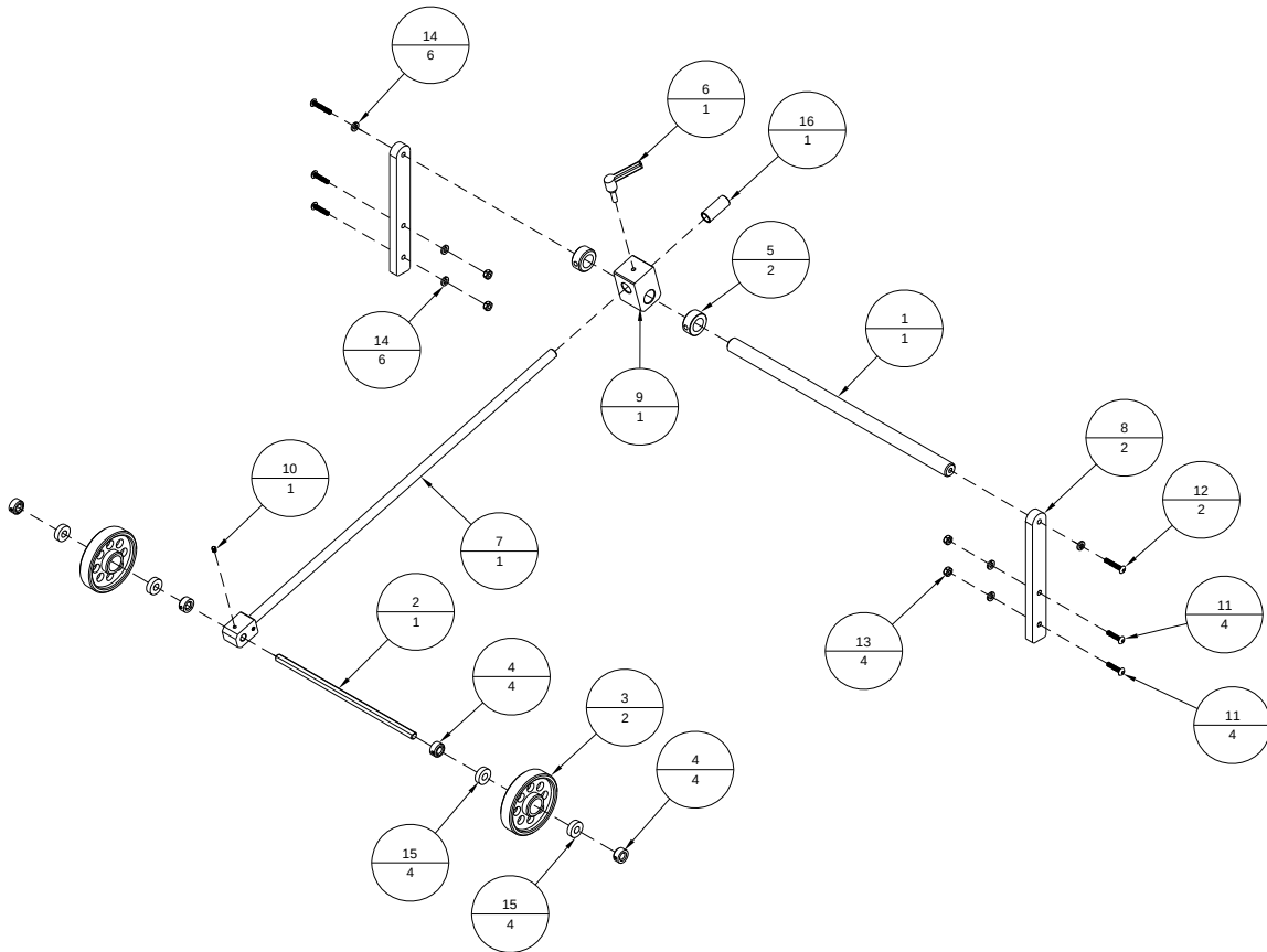
Figure A-18: 100180A - Inline Roller Bar Assembly
