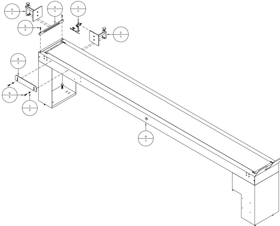
Figure A-5: BK1612SB - Conveyor, 12', Solid Belt, Right Angle
