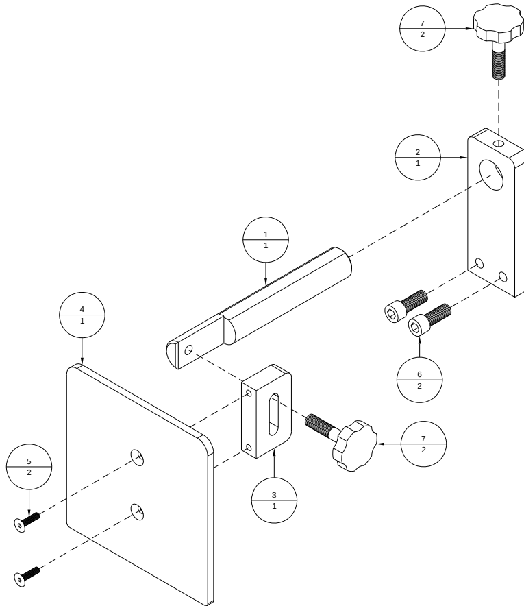
Figure A-21: 330136A - Side Plate Knockdown Assembly
