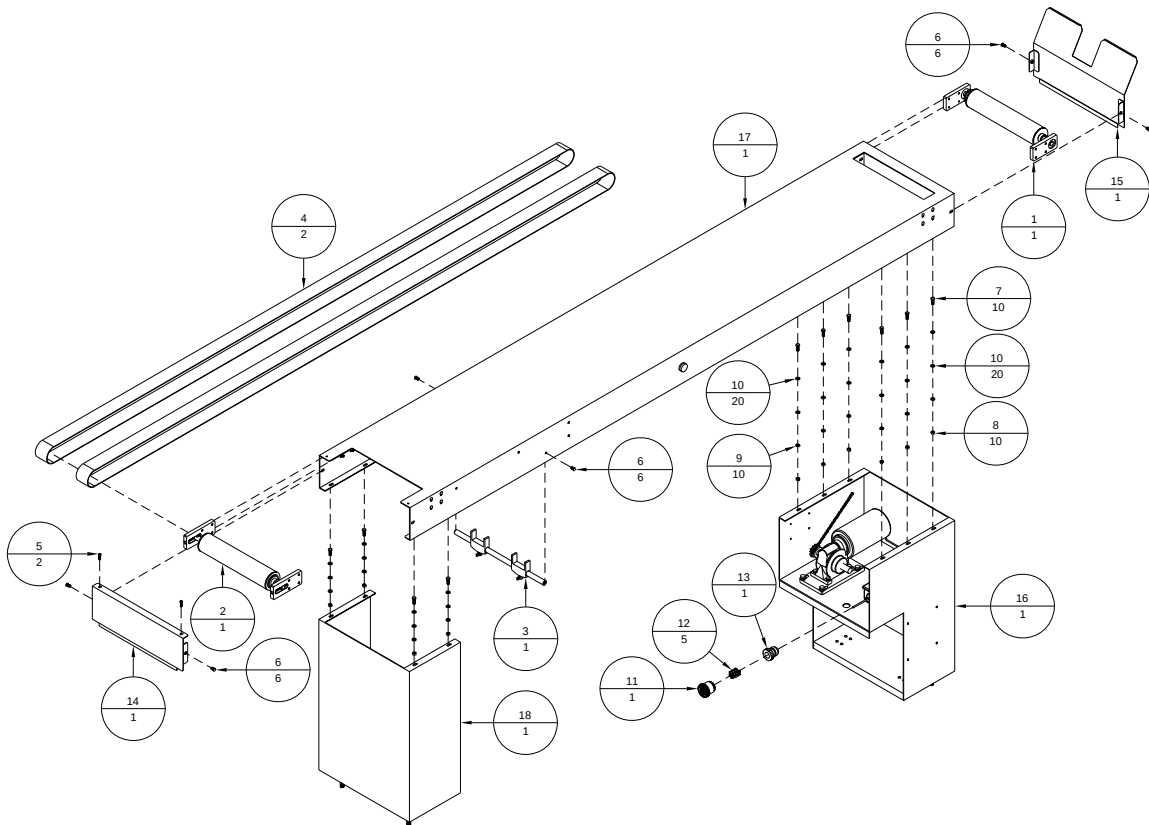
Figure A-9: BK1608A - Conveyor Assembly, 8', Twin Belt
