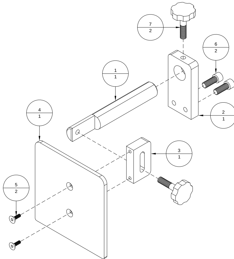
Figure A-20: 330135HA - End Plate Knockdown Assembly
