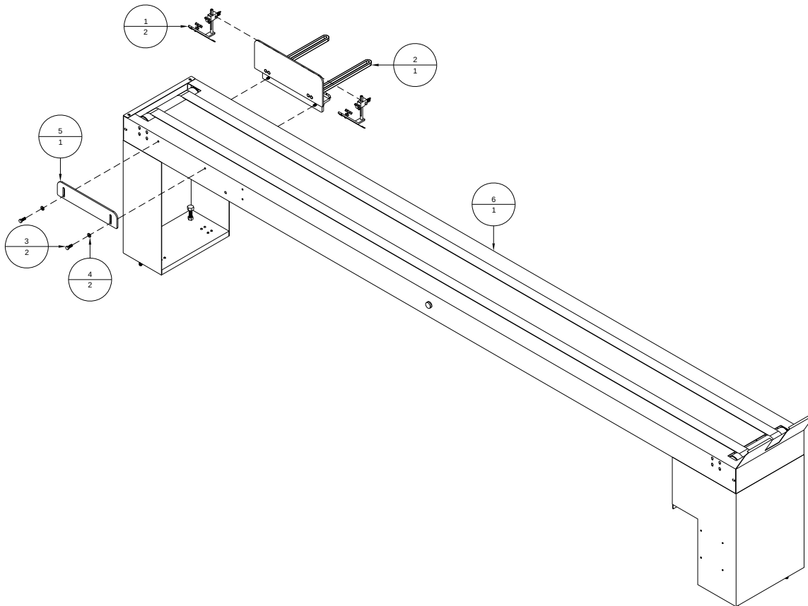
Figure A-7: BK1612TB - Conveyor, 12' Twin Belt, Right Angle
