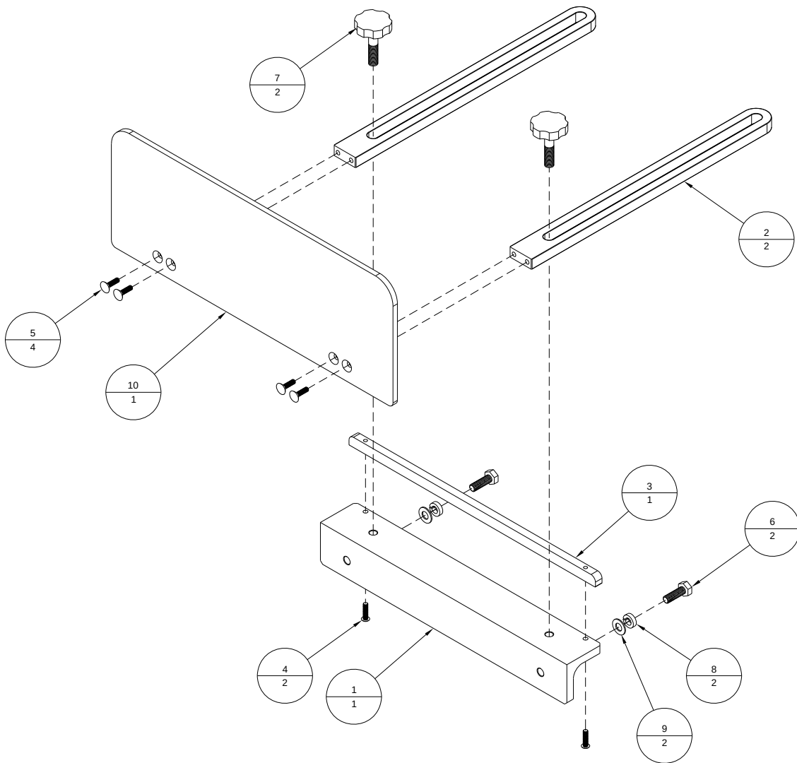
Figure A-22: 330141A - Material Guide Assembly
