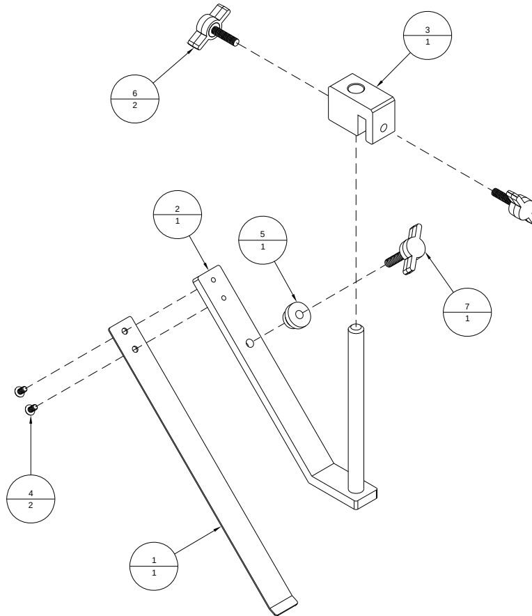
Figure A-19: 212150A - Knockdown Arm Assembly
